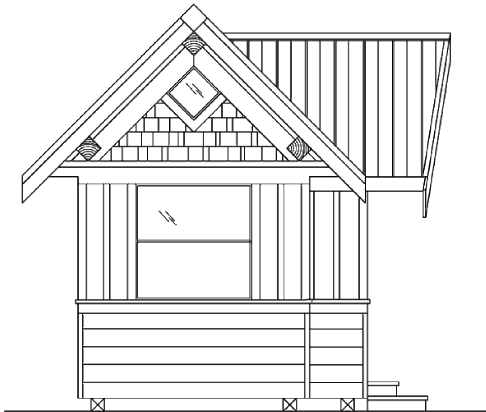
LEFT VIEW
